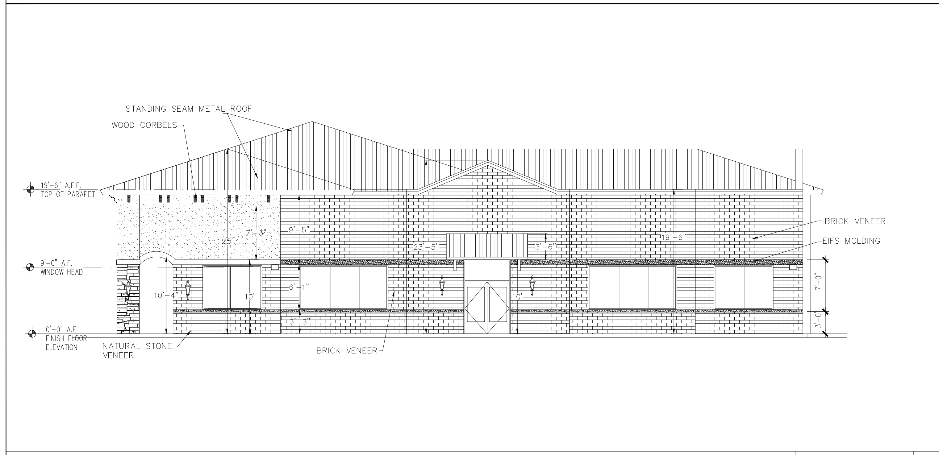
SOUTH BUILDING ELEVATION
