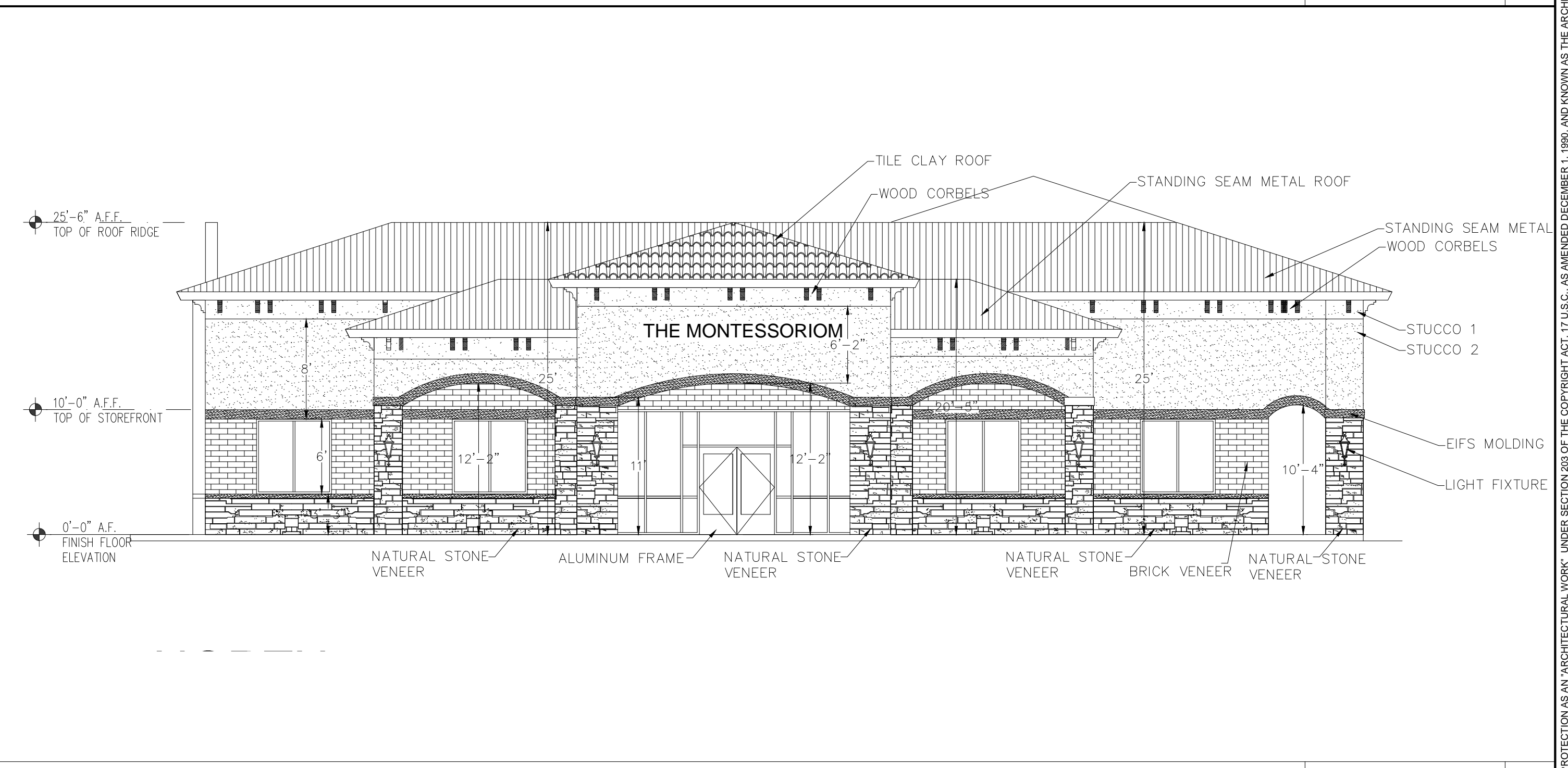
NORTH BUILDING ELEVATION
