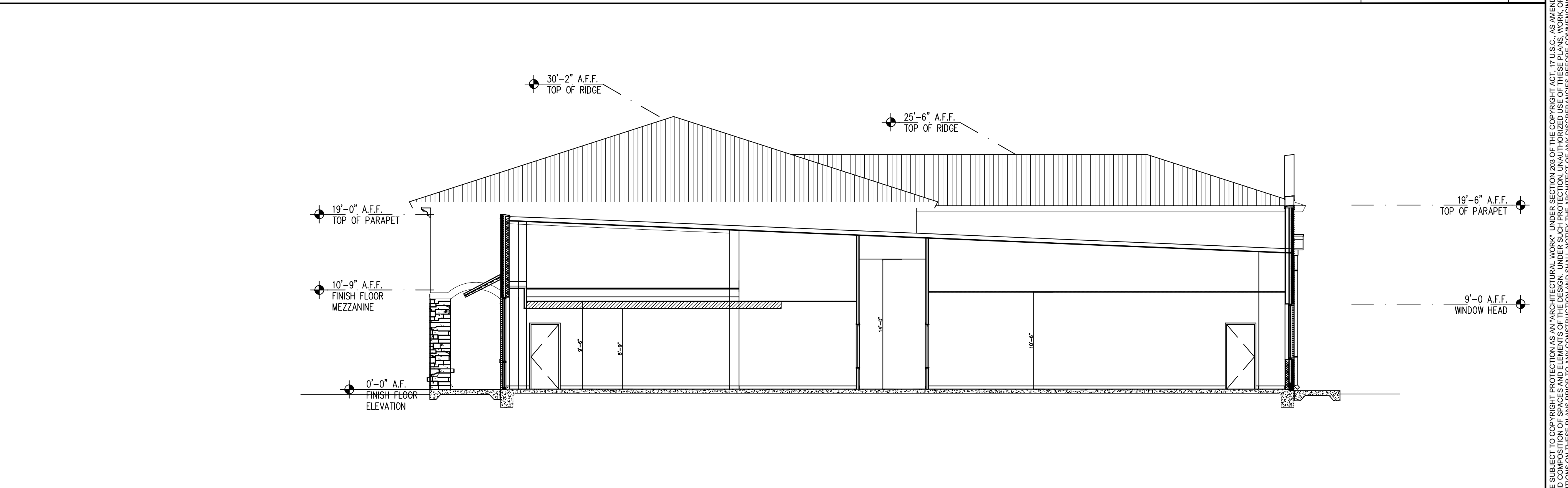
BUILDING SECTION B
