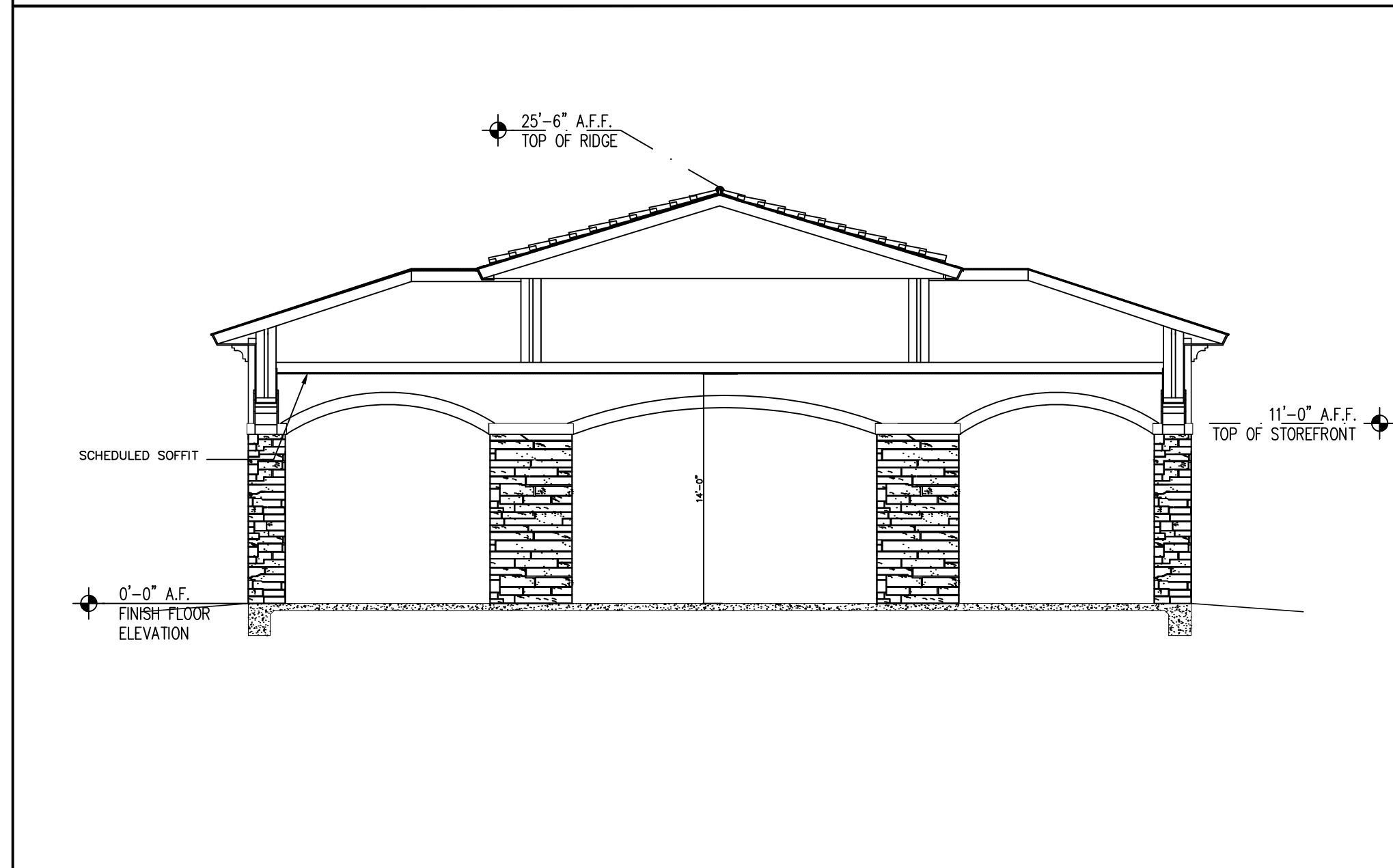
BUILDING SECTION C
