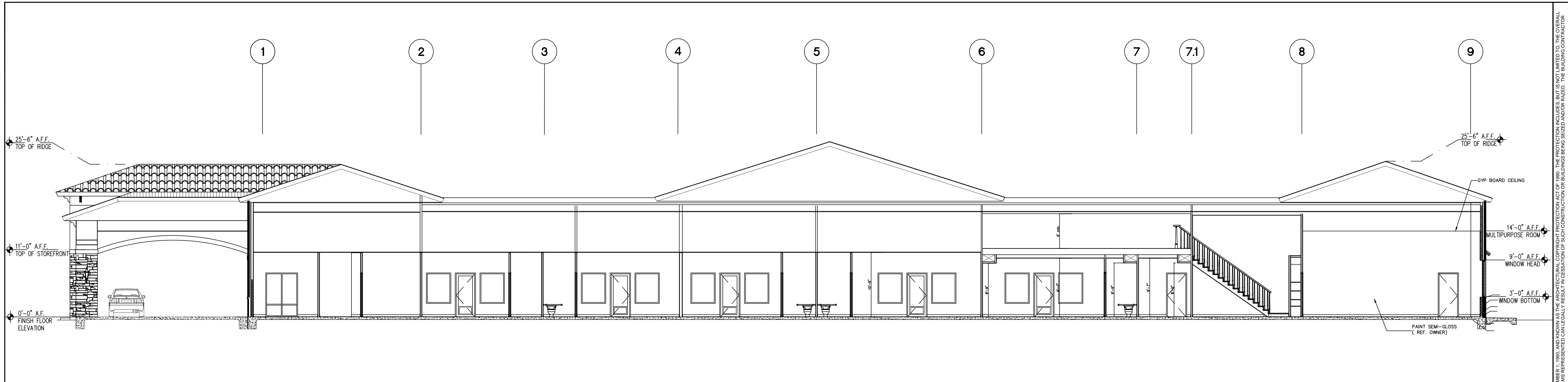
BUILDING SECTION A
